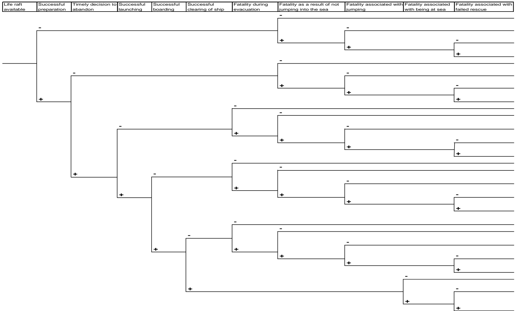
Overboard Life Raft Event Tree
