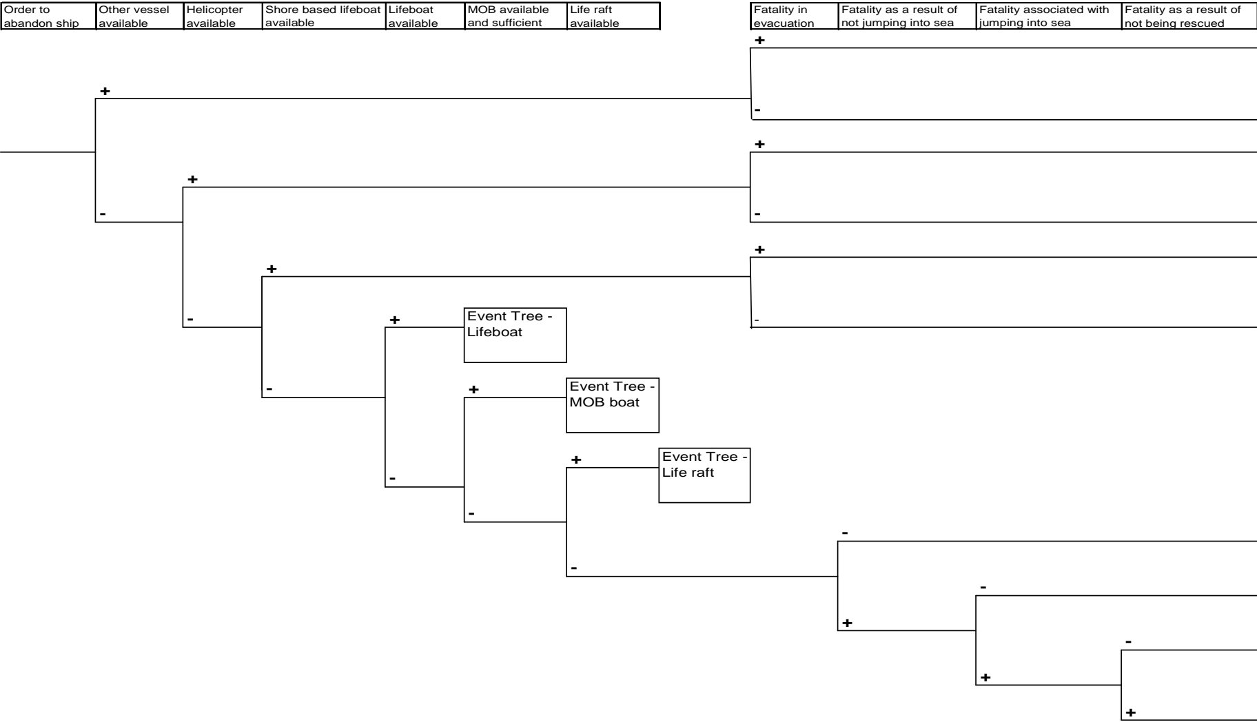
Abandoning Event Tree
