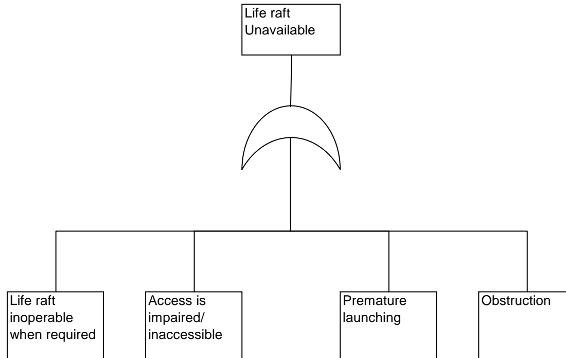
Overboard Life Raft Fault Tree
