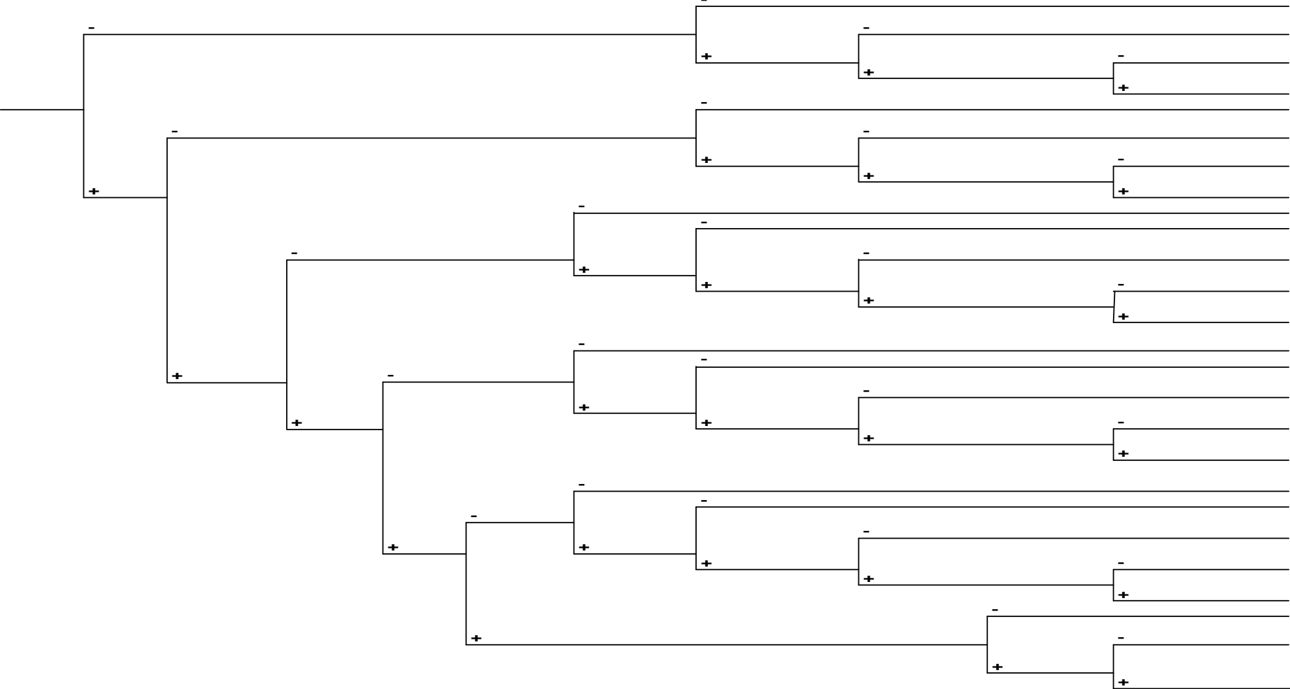
Launched Life Raft Event Tree
