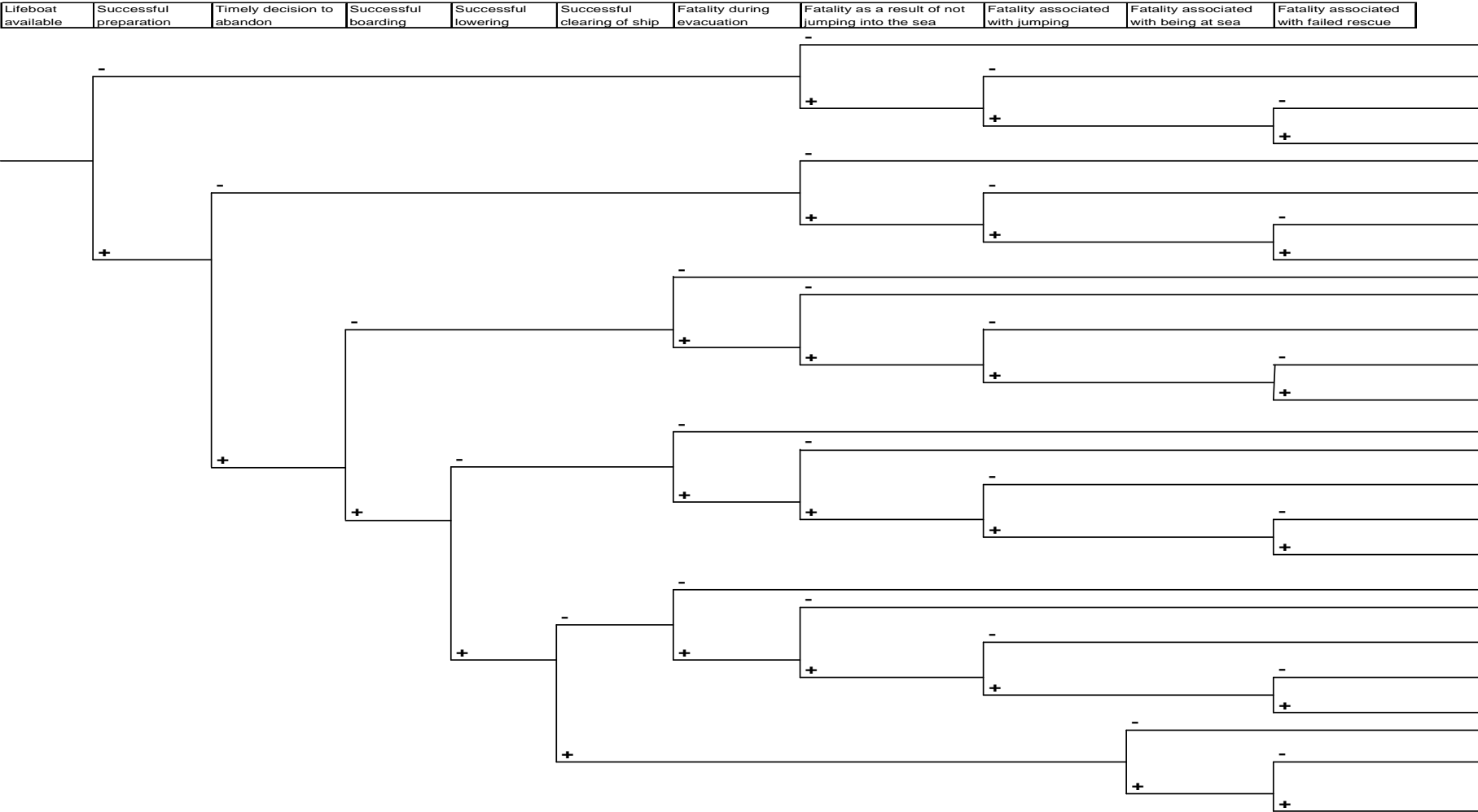
Lifeboat Event Tree
